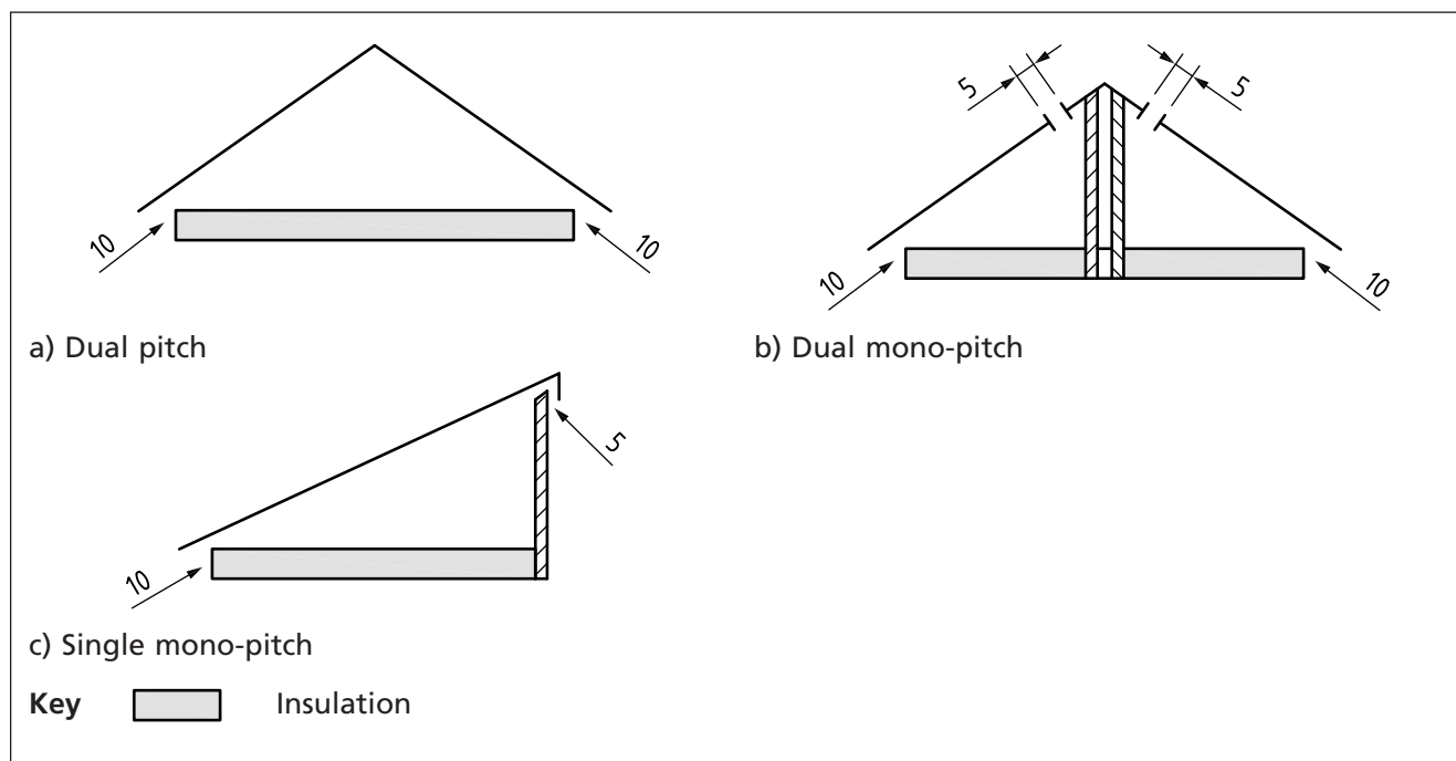
Figure 2 Cold pitched roofs with pitch \geq 15^\circ
