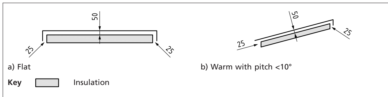
Figure 5 Flat roofs and warm roofs with pitch <10^\circ
